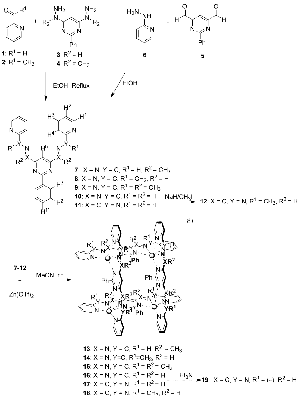
Scheme 1. Synthesis of the ligands 7–12 and of the [2 \times 2]\text{Zn}^{2+}_4 grid-type complexes 13–18.
