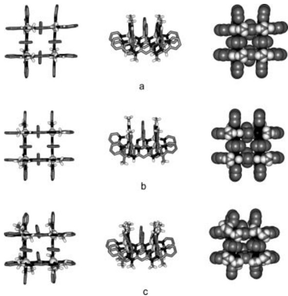
Figure 1. Crystal structure of the [2 \times 2]\text{Zn}_4^{2+} grid complexes: a) 13 , b) 14 , c) 15 : top view (left), side view in stick representation (center) and space-filling representation (right). The \text{Zn}^{2+} ions are shown as spheres.
