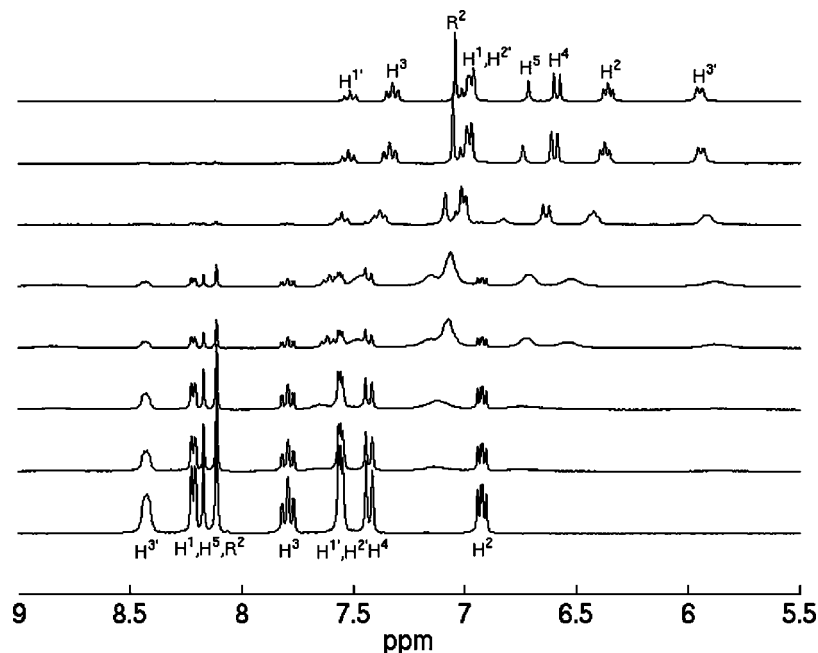
Figure 4. ^1H NMR of grid complex 17 with triethylamine in [D_6] DMSO. From bottom to top, the ratio Et_3N/17 is 0.0, 1.0, 2.0, 4.3, 5.0, 6.8, 9.3, 11.9.
